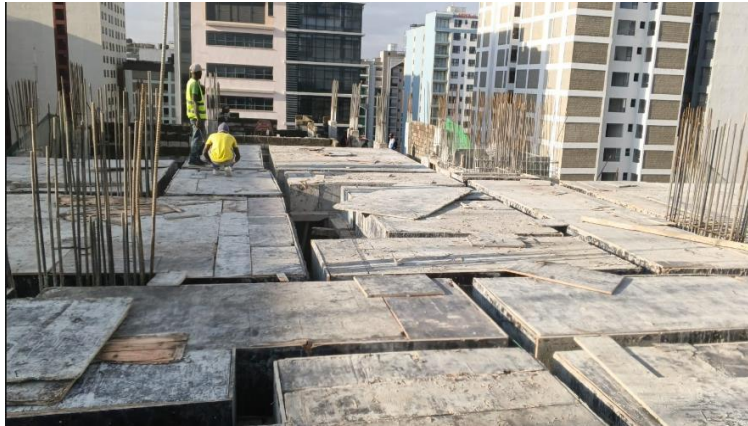
11th floor suspended slab shutter
